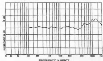
FIGURE 1 — Frequency Response
